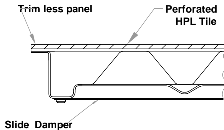
PARTIAL SECTION VIEW
